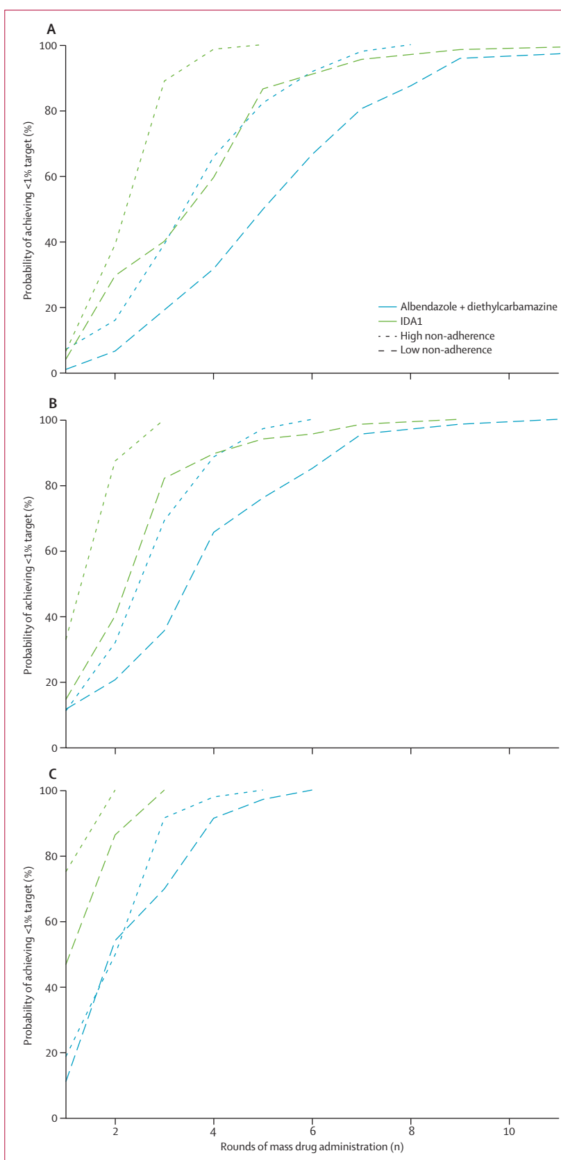
Figure 3: Relative effects of population coverage and systematic non-adherence Plots show the probability of achieving target prevalence (<1%) with two-drug (blue line) and triple-drug (green line) regimens with high and low systematic non-adherence (dashed lines) when population coverage is (A) poor (55%), (B) standard (65%), and (C) high (75%). IDA1=ivermectin, diethylcarbamazine, and albendazole as efficacious as two-drug regimen and 100% worm sterilisation.
